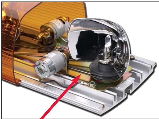
The belt-driven rotator assembly, provides a quiet and reliable lighting source.
